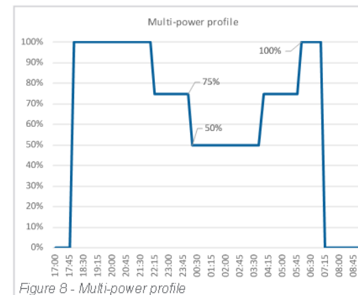
Figure 8 - Multi-power profile
