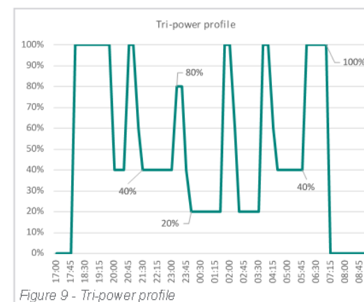
Figure 9 - Tri-power profile
