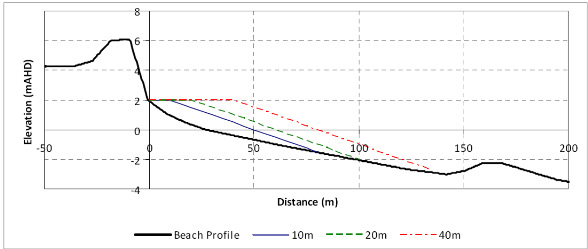
Figure 2-5 Measured Beach Profile and 10m, 20m and 40m Design Berm Profiles
