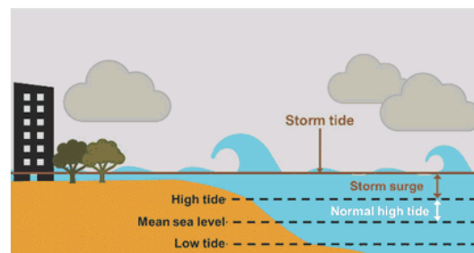
Figure 1. Storm tide inundation
