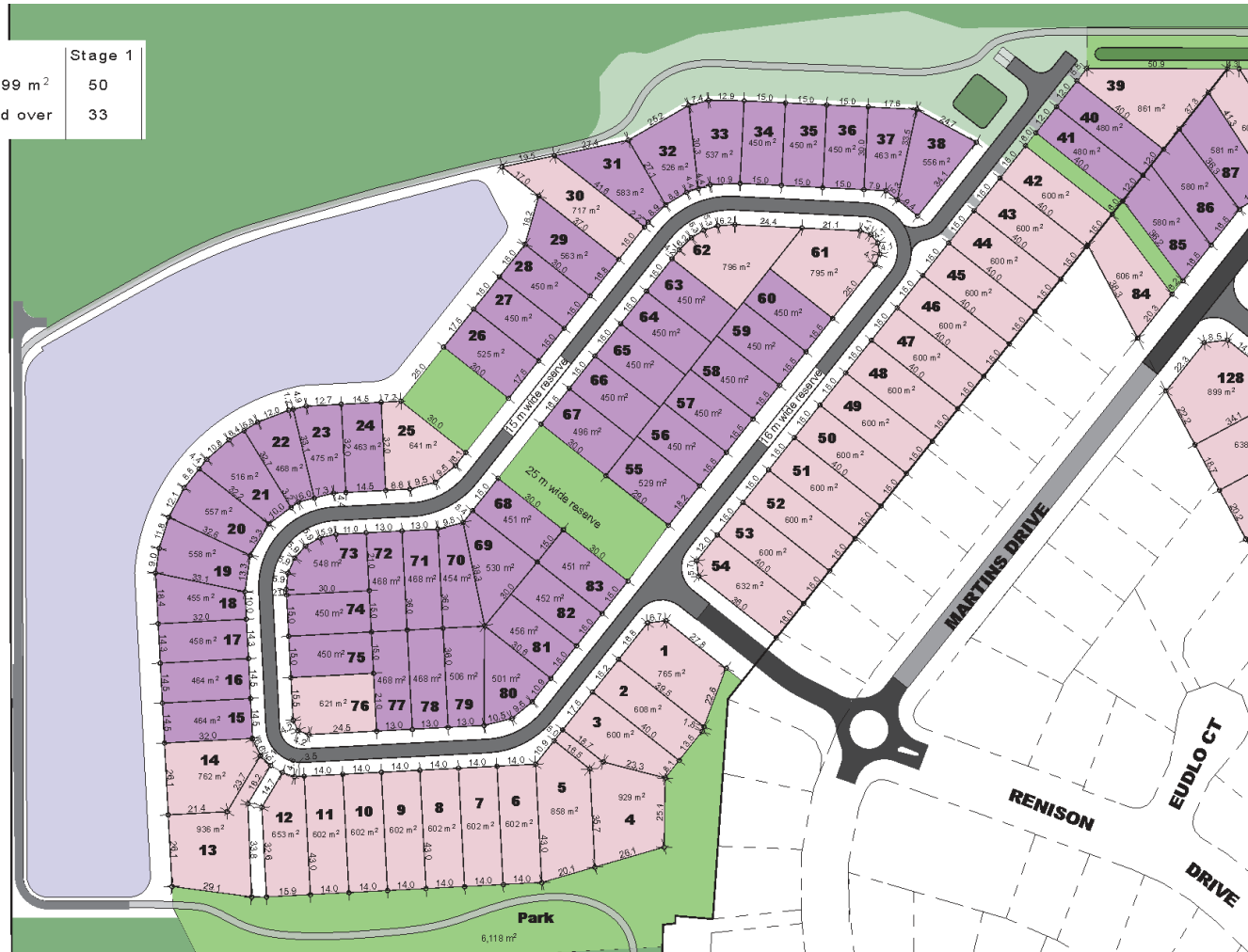
Dimensioned Lot Plan
