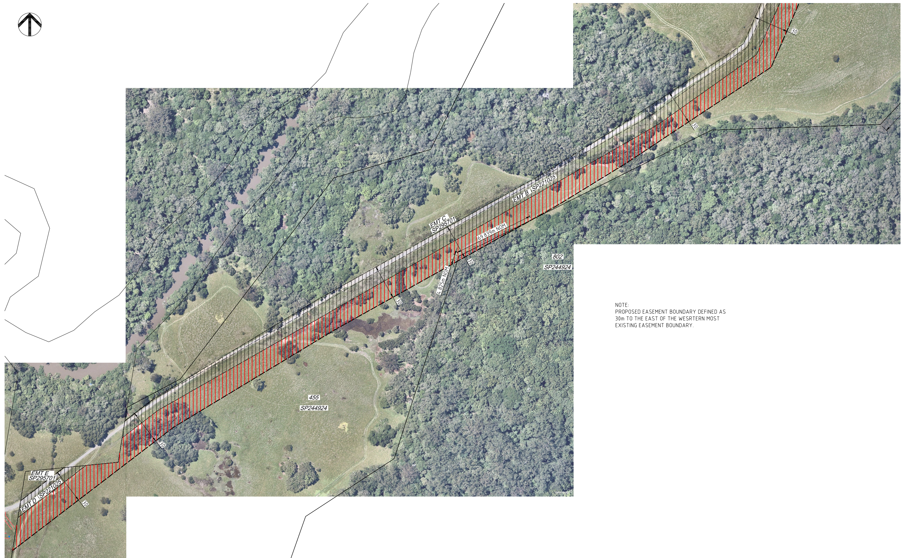
PROPOSED PIPELINE EASEMENT SCALE 1:1000
