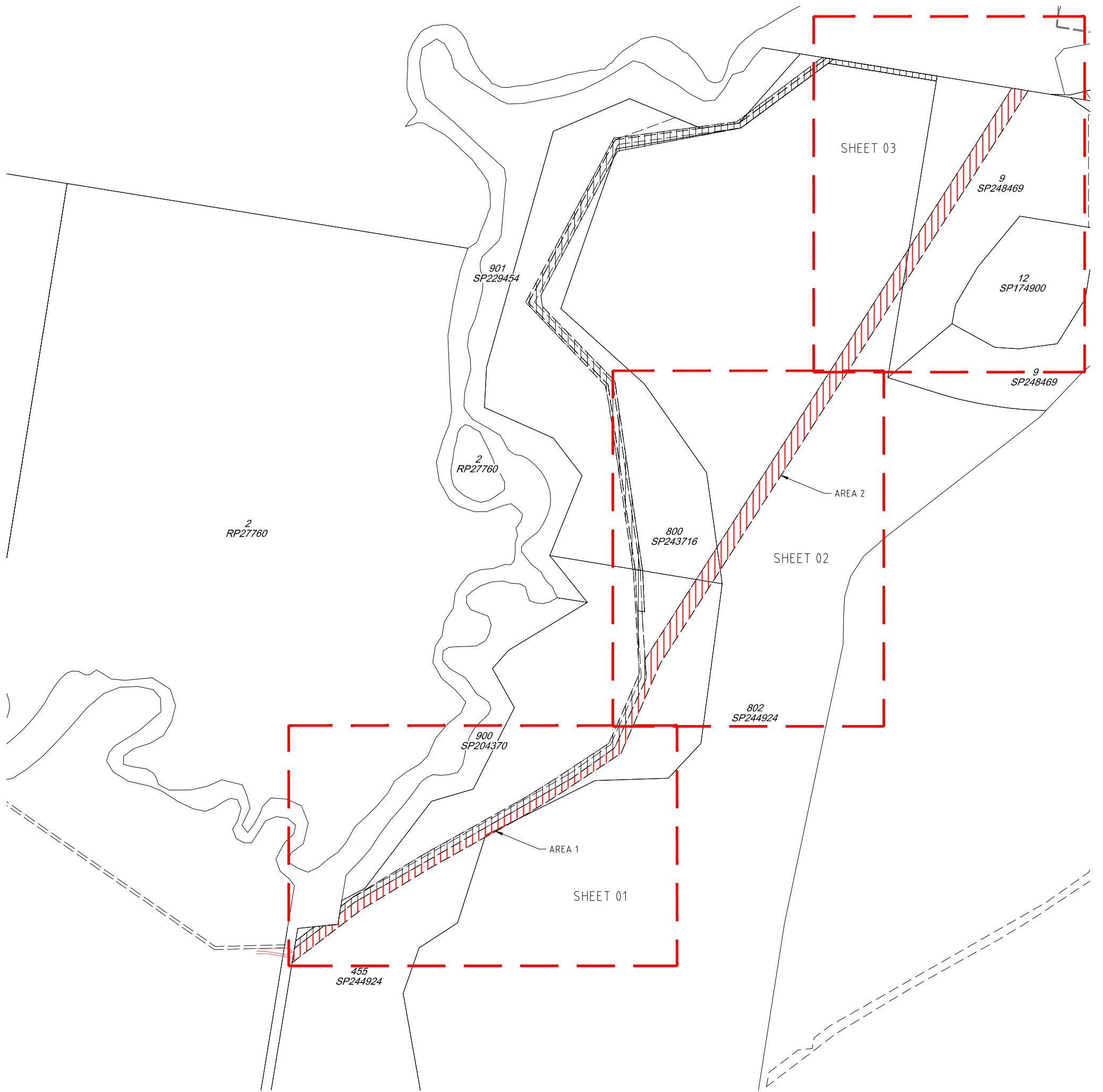
PROPOSED PIPELINE EASEMENT SCALE 1:4000
