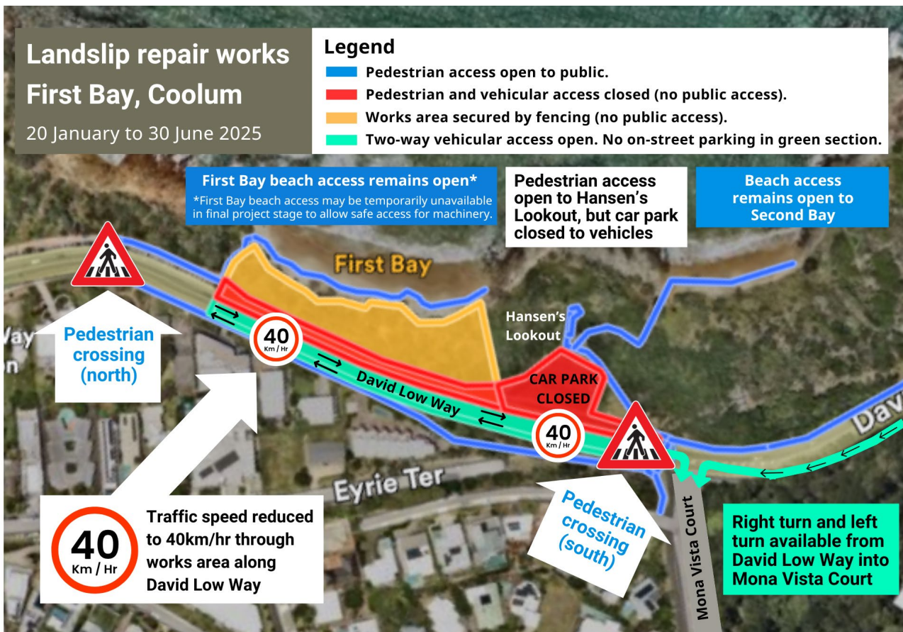
Figure 1: Landslip Repair - First Bay, David Low Way, Coolum
