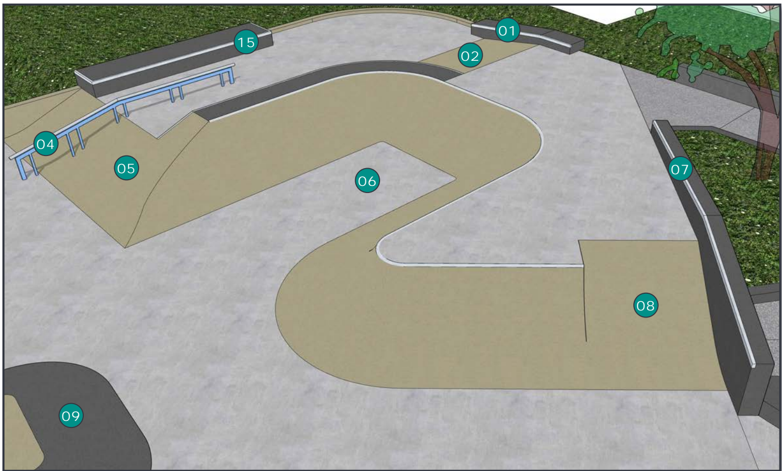
PERSPECTIVE C - LOOKING SOUTH
