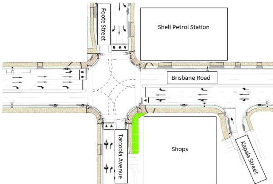
Figure 2. New signalised intersection
