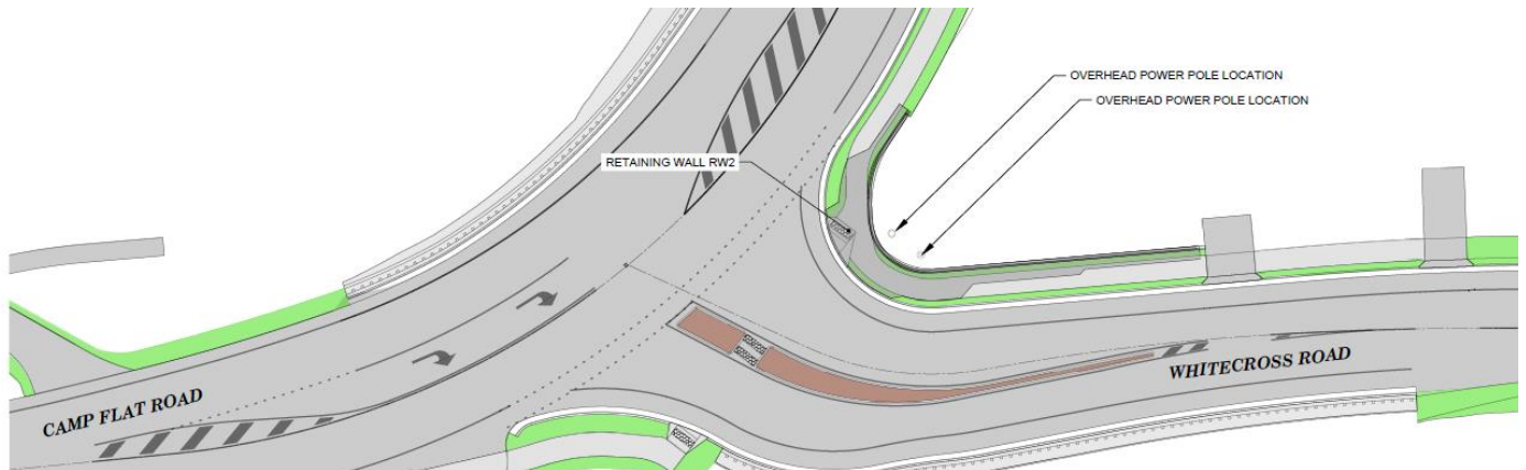
Figure 2: Camp Flat and Whitecross Road Retaining Wall Design
