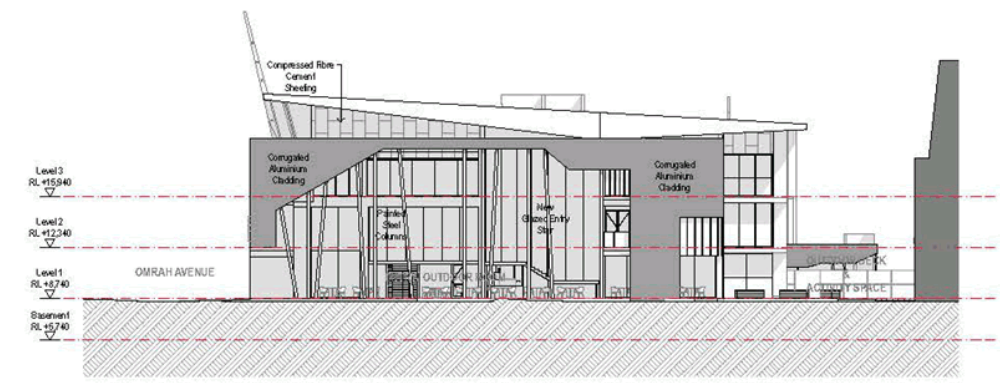
2 EAST ELEVATION 1:200
