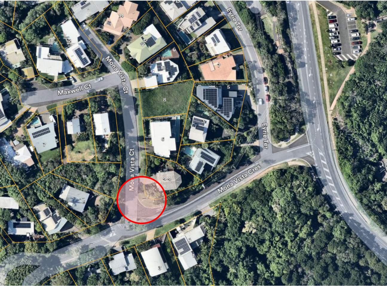
Figure 1: Mona Vista Court stormwater pit replacement location
