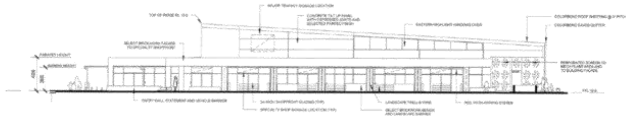
NORTH EAST ELEVATION - DAVID LOW WAY 1:200
