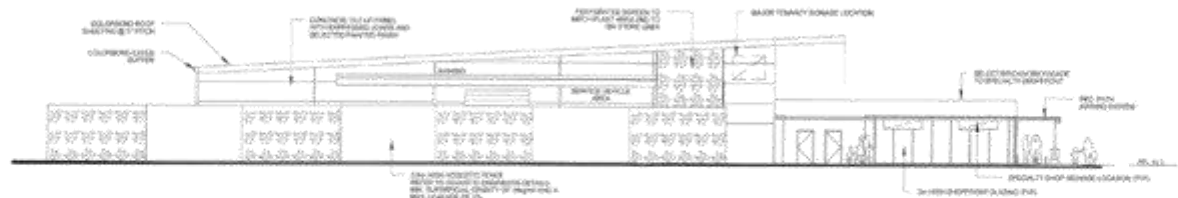
SOUTH WEST ELEVATION - RUFUS STREET
