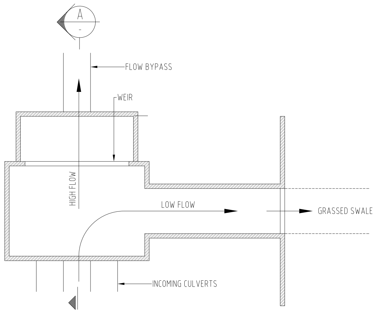
PLAN INDICATIVE DIAGRAM FOR HIGHFLOW BYPASS ARRANGMENT NOT TO SCALE
